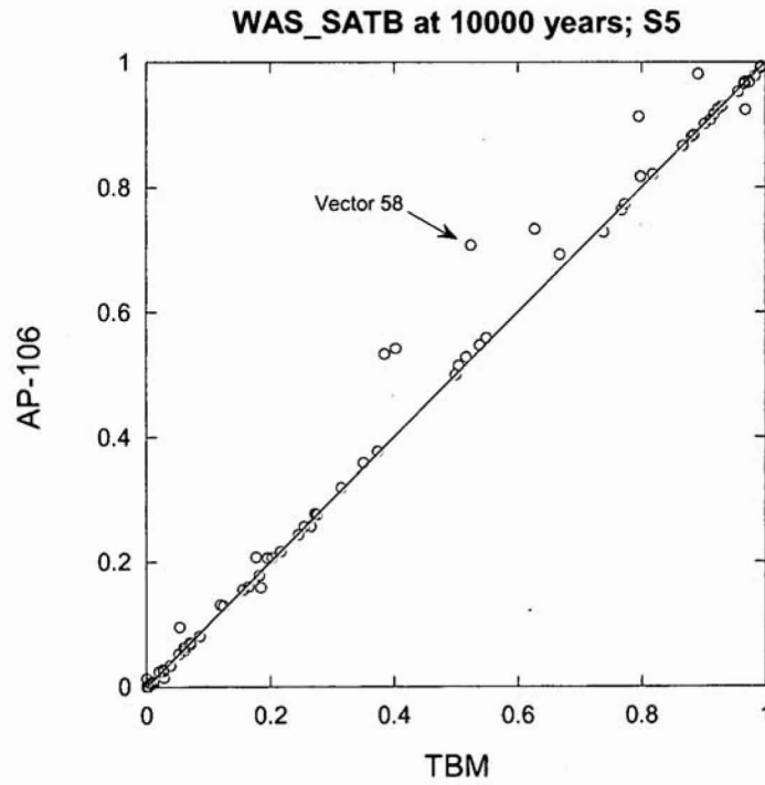
Figure 45. Scatter plot of brine saturation in the intruded panel at 10,000 years; S5
