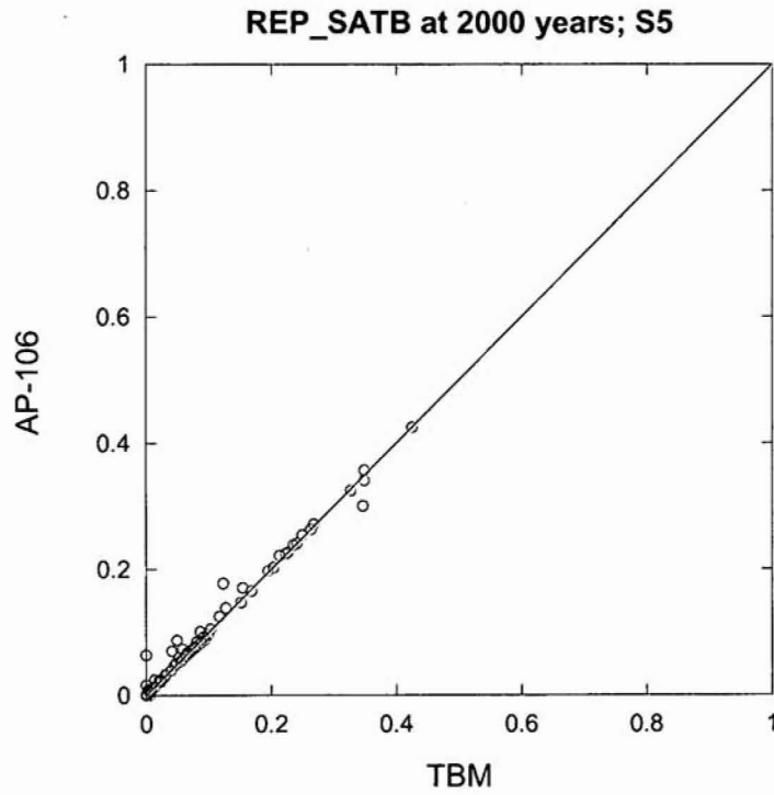
Figure 49. Scatter plot of brine saturation in the rest of repository at 2,000 years; S5
