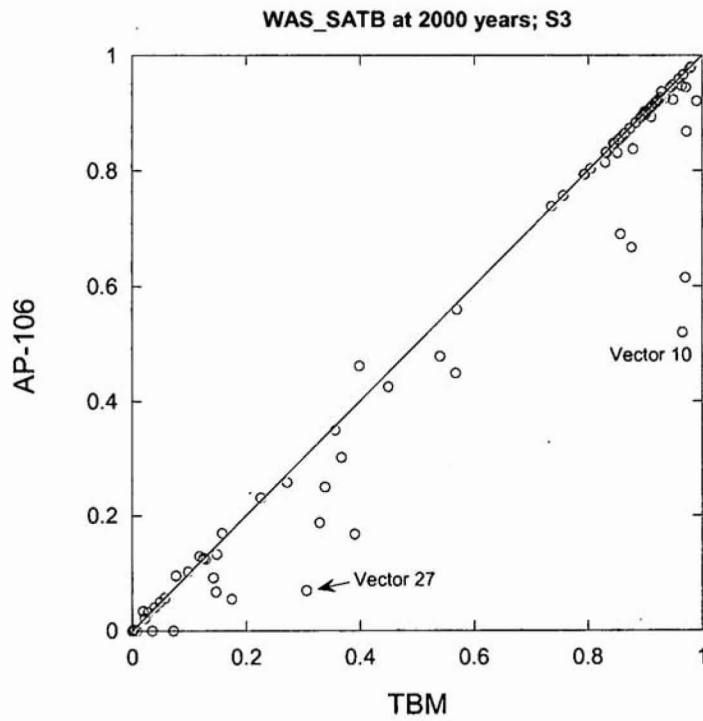
Figure 36. Scatter plot of brine saturation in the intruded panel at 2,000 years; S3
