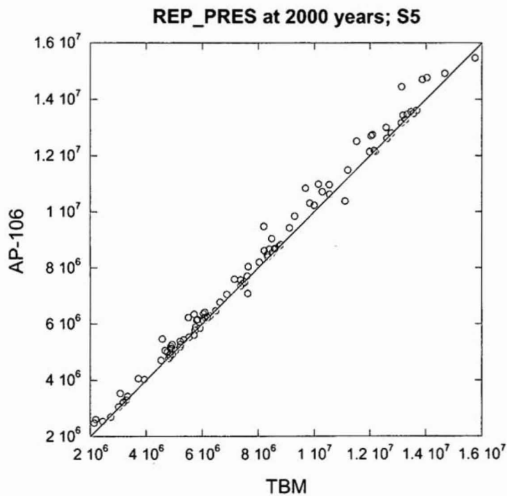
Figure 23. Scatter plot of pressure in the rest of repository at 2,000 years; S5
