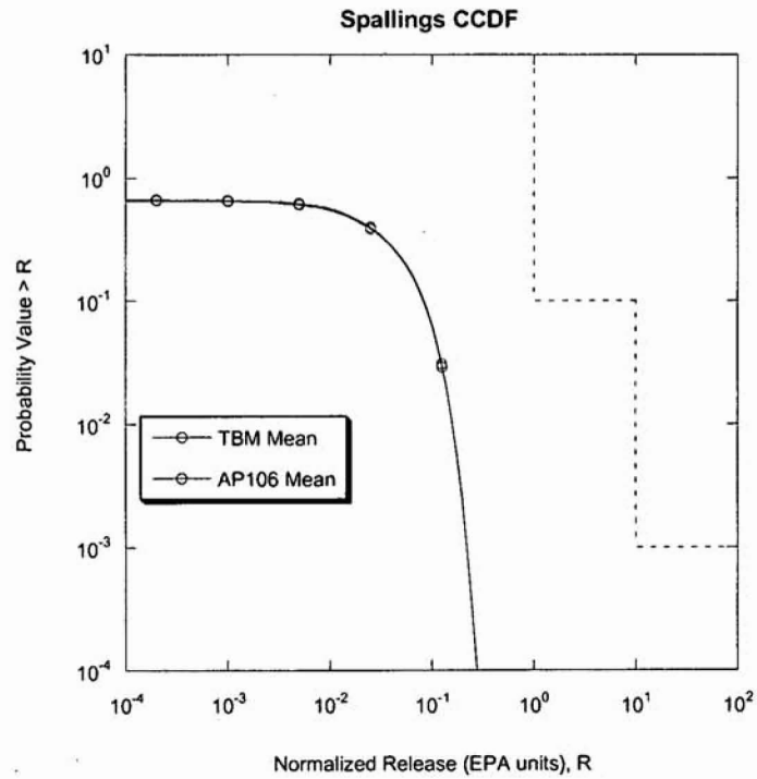
Figure 52. Mean spallings CCDF results from AP106 and TBM.
