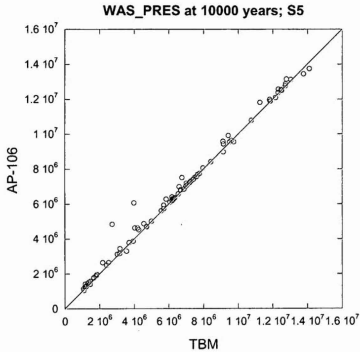
Figure 21. Scatter plot of pressure in the intruded panel at 10,000 years; S5
