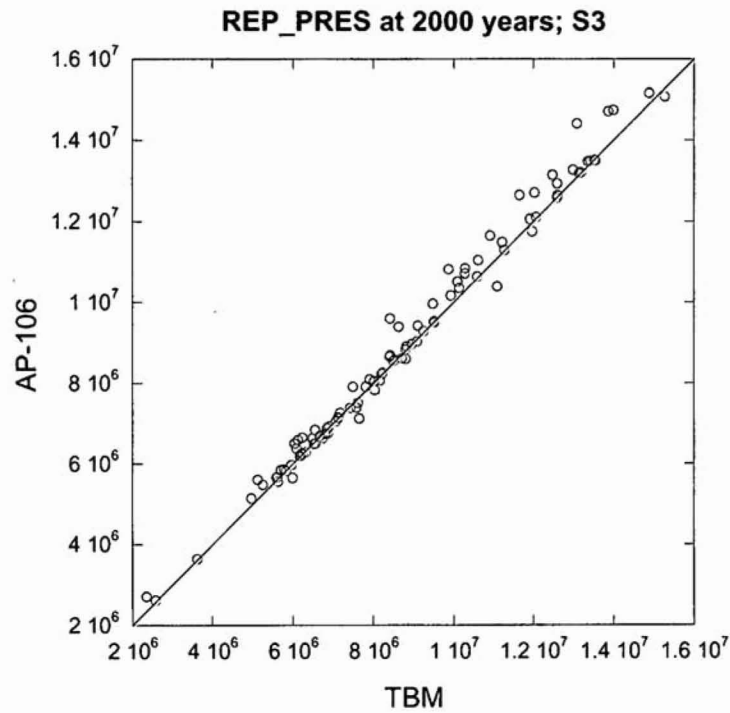
Figure 16. Scatter plot of pressure in the rest of repository at 2,000 years; S3
