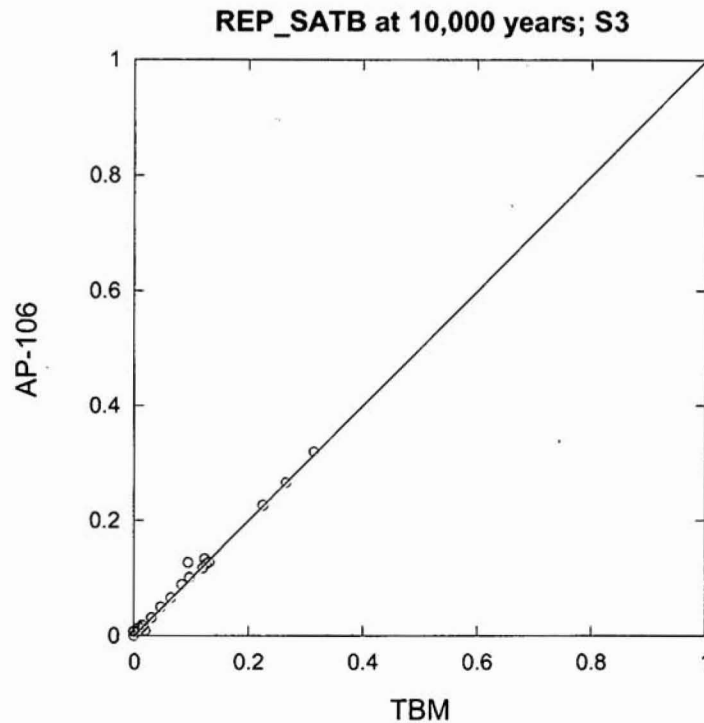
Figure 42. Scatter plot of brine saturation in the rest of repository at 10,000 years; S3
