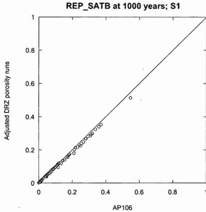
Figure 65. Scatter plot of brine saturation in the rest of repository at 1,000 years; AP106 S1 vs. S1_P2
