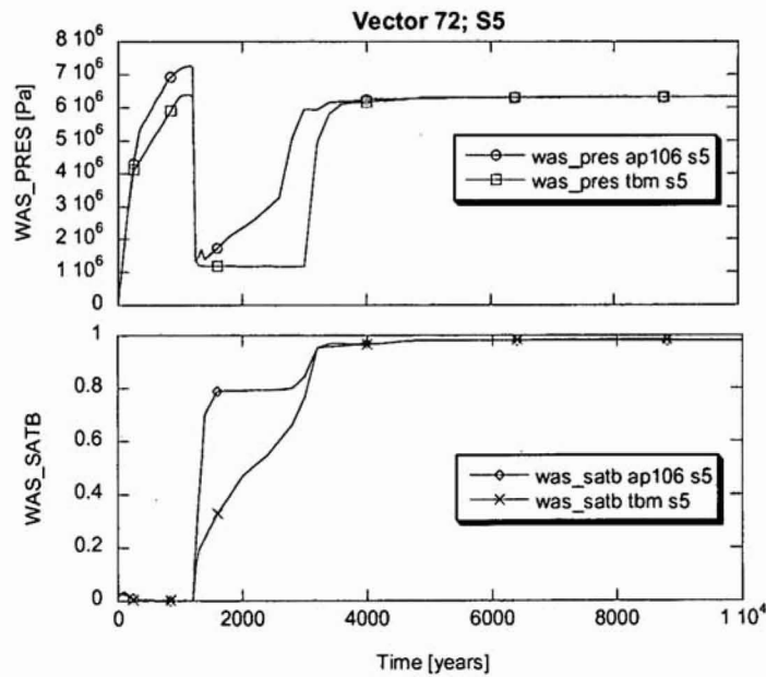
Figure 47. Detailed plot of pressure and brine saturation (separate plots for clarity) time histories for vector 72; S5
